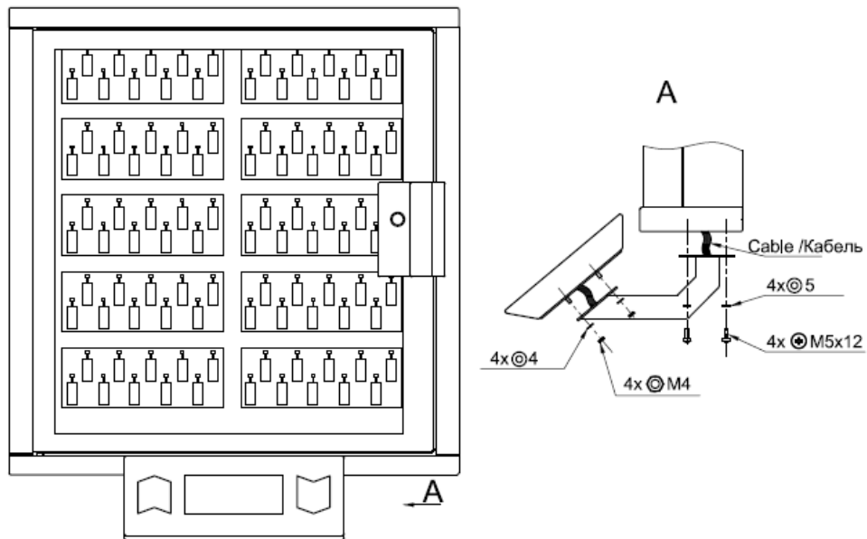
Bottom installation
