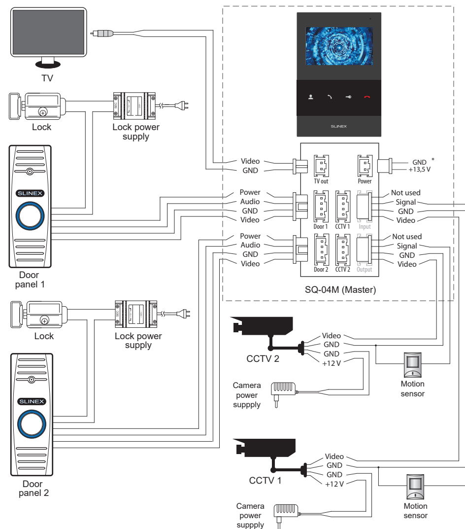
Diagram 1. SQ-04M door panels, cameras, locks and TV connection.
